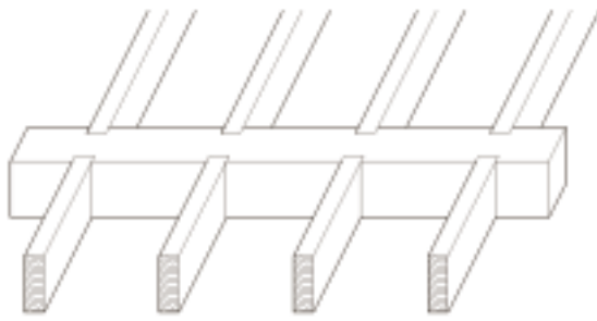
JOISTS FRAMING INTO NOTCH BEAM
