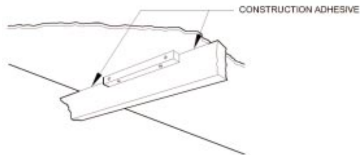
FIGURE 3 APA PLUMBER STRIP
