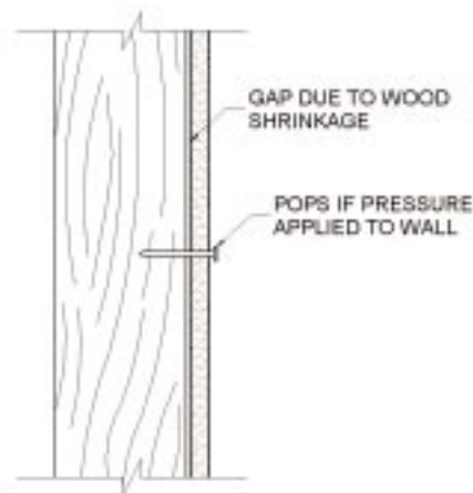
NAIL POPS
