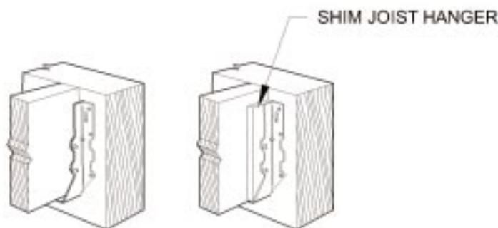
SHIM JOIST HANGER
